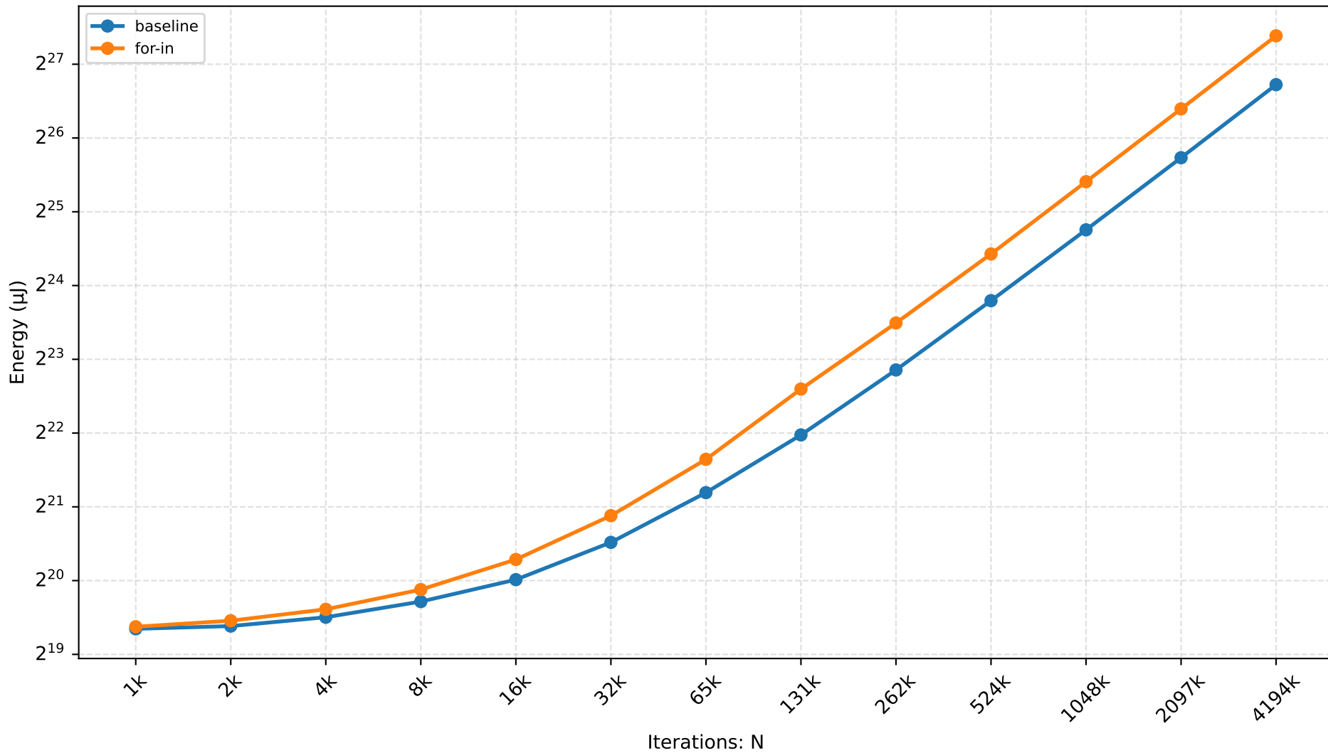
XS — object-iteration Scaling
