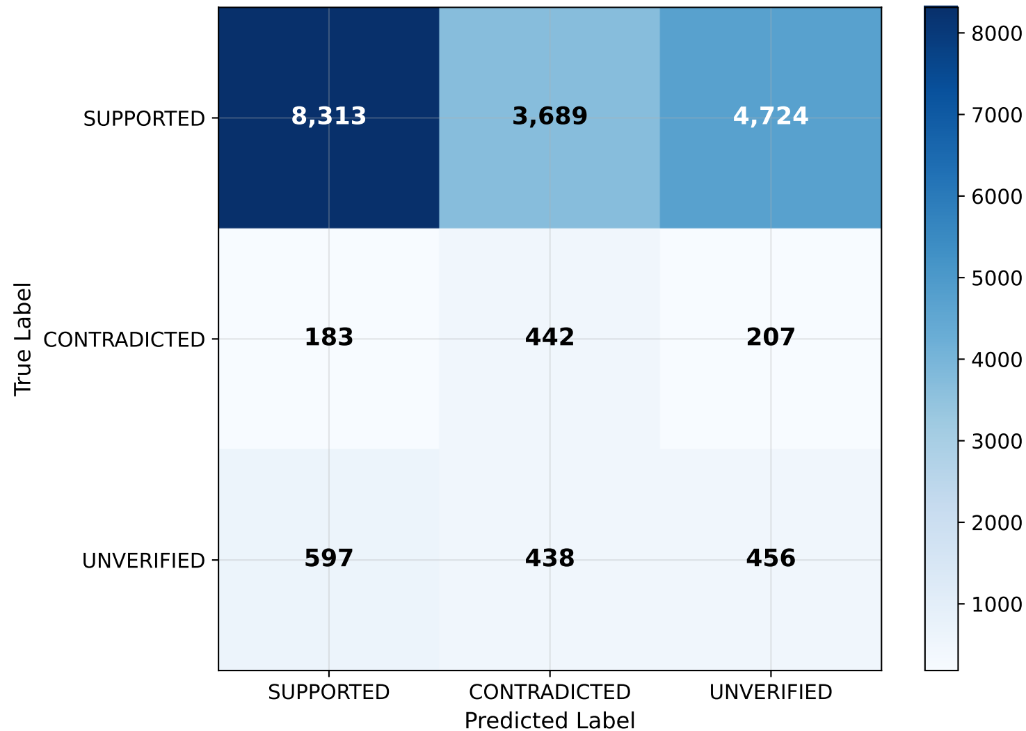
TRUVI-EV Confusion Matrix (Validation Set)
