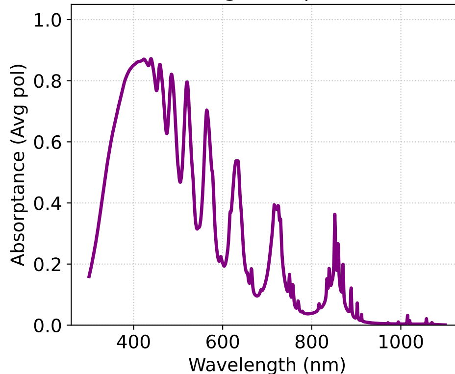
Grating Absorptance
