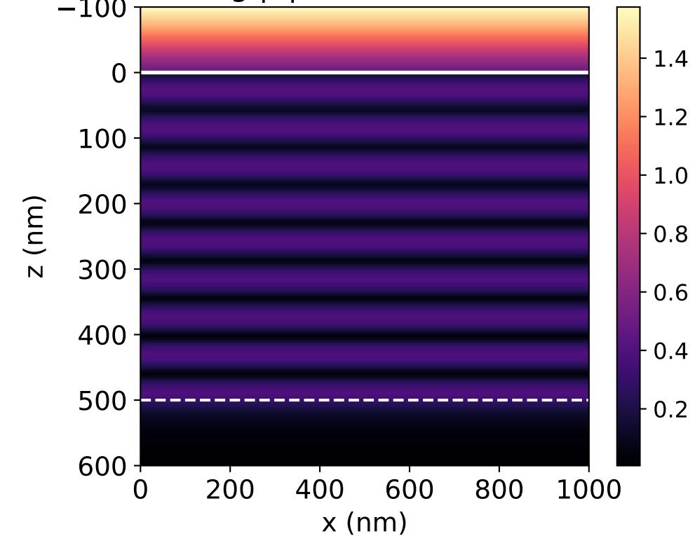
Avg |E| field at 495 nm
