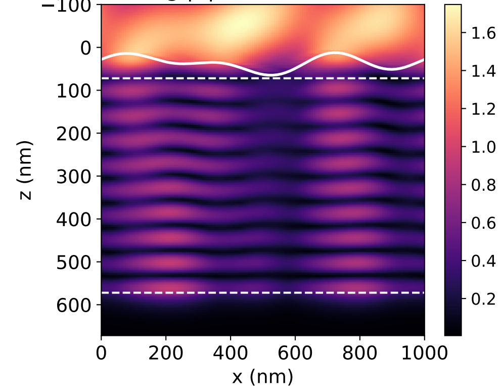
Avg |E| field at 495 nm
