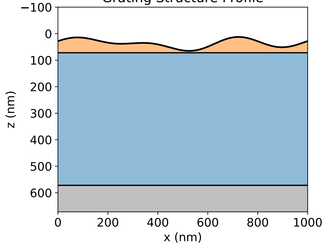
Grating Structure Profile
