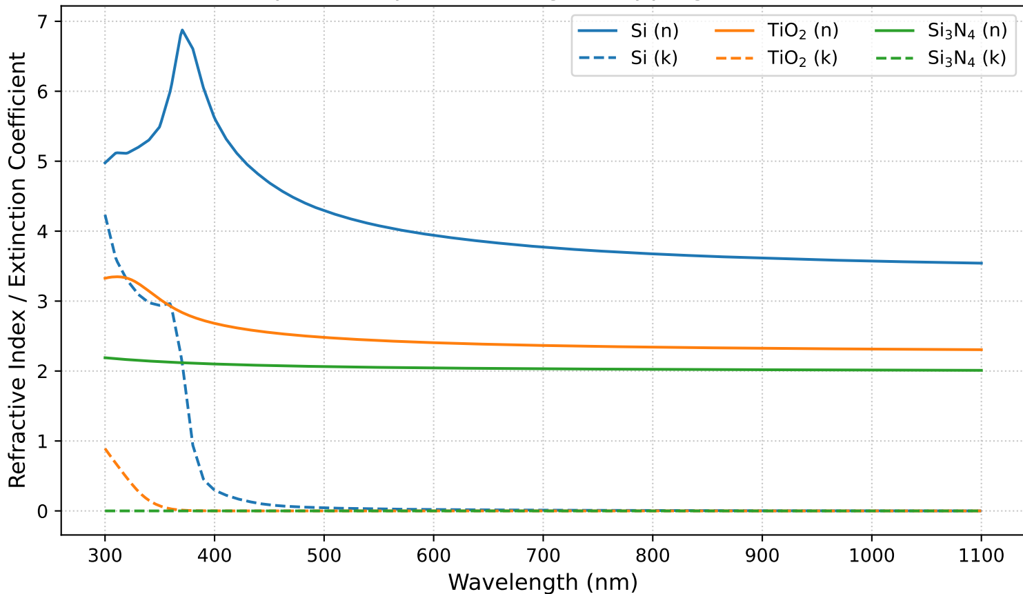
Optical Properties of Light-Trapping Materials
