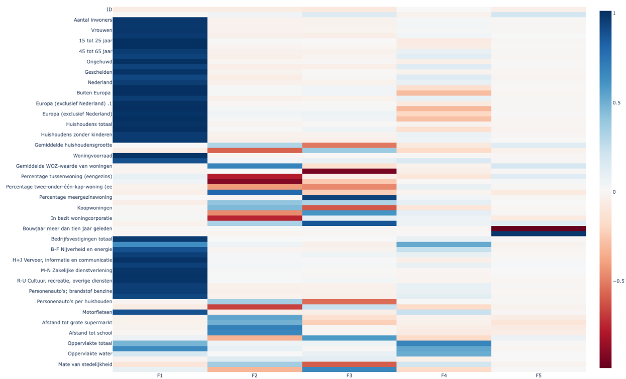
FA Loadings Heatmap
