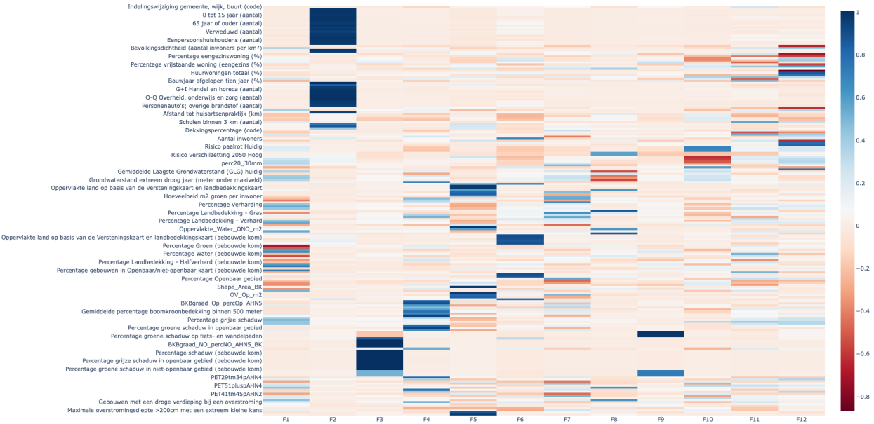
FA Loadings Heatmap
