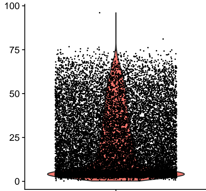
percentMT_6wk
