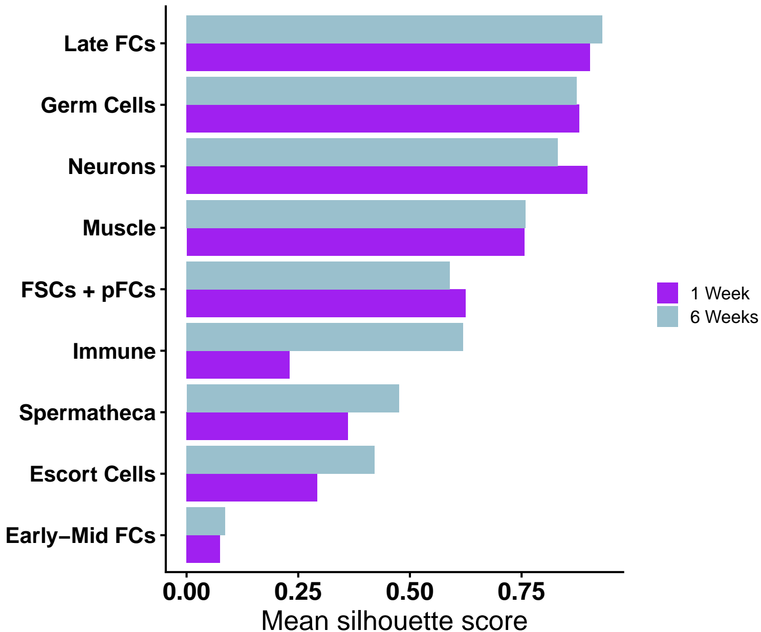
Cluster separability within each age
