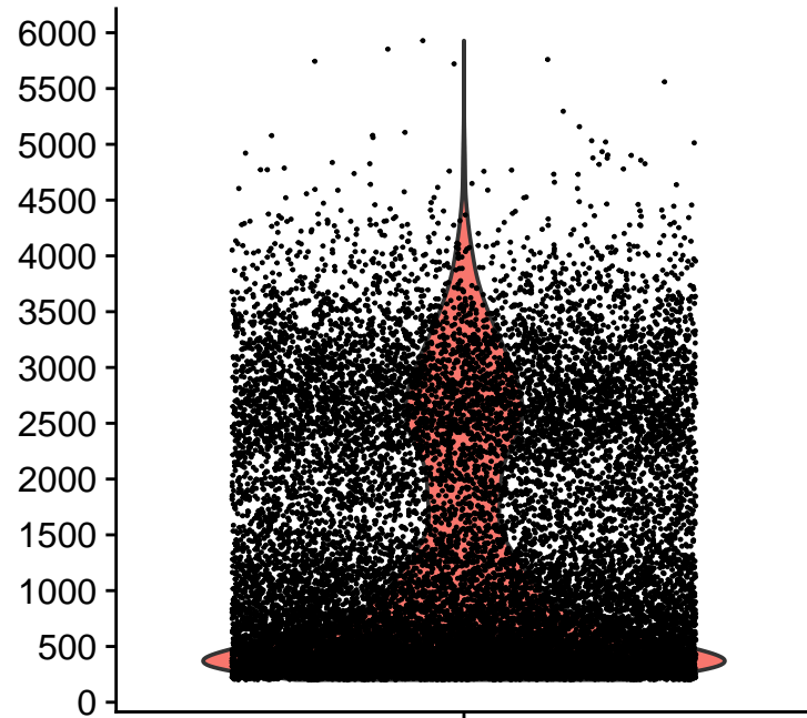
nFeature_6wk
