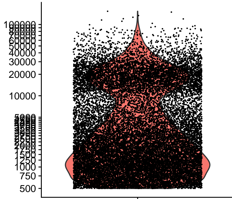
nCount_6wk
