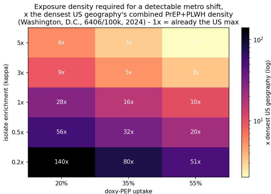
Figure B. Metro level. Exposure density required for a detectable shift, as multiples of the densest US geography's combined PrEP+PLWH density (Washington, D.C., 6 406/100 000 adult males, 2024). 1× is already the national maximum; the best cell needs \approx 2\times it.
