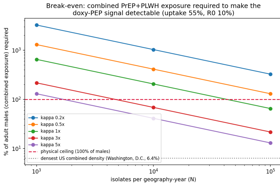
Figure C. Break-even in proxy-free units. Share of all adult males under combined PrEP+PLWH exposure required for detection versus isolates per geography-year, by enrichment \kappa . Every curve sits above D.C.'s observed combined density (6.4%) and, under realistic isolate volumes, above the 100%-of-males physical ceiling.
