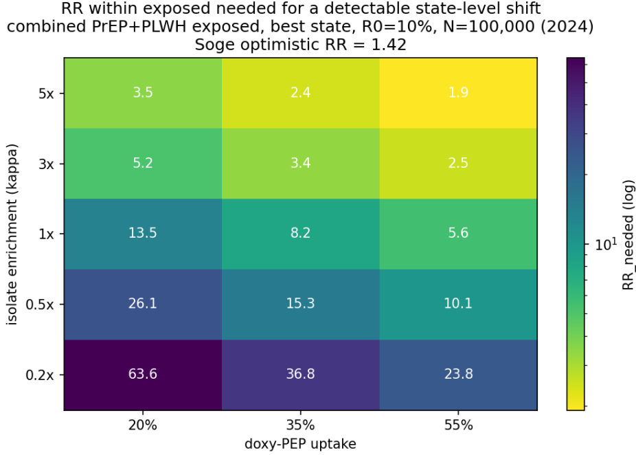
Figure A. State level. Within-exposed RR required for a detectable state-level shift in tetracycline non-susceptibility, over doxy-PEP uptake \times isolate enrichment (combined PrEP+PLWH exposed, best state, R_0 = 10\% , N = 100\,000 /state-year, 2024). Every cell exceeds the optimistic benchmark RR = 1.42 (minimum \approx 1.9 ).
