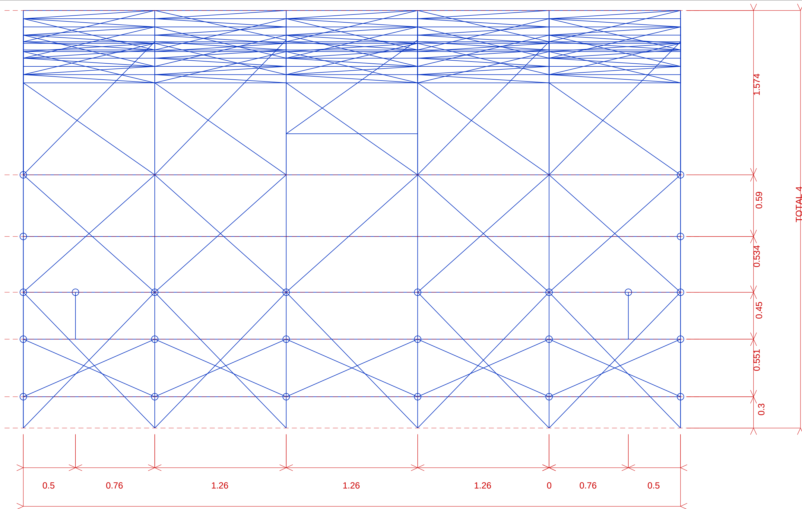
FRONT VIEW
