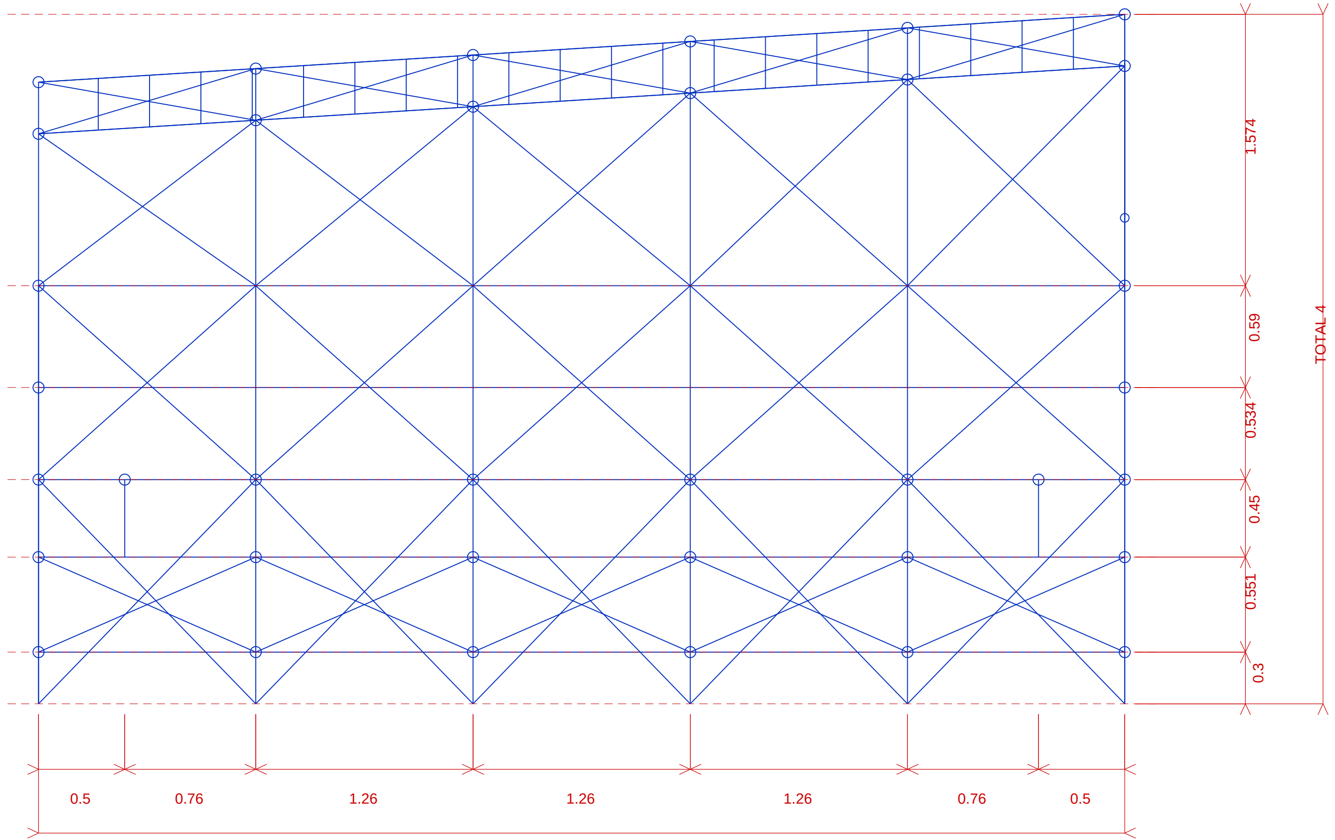
SIDE VIEW
