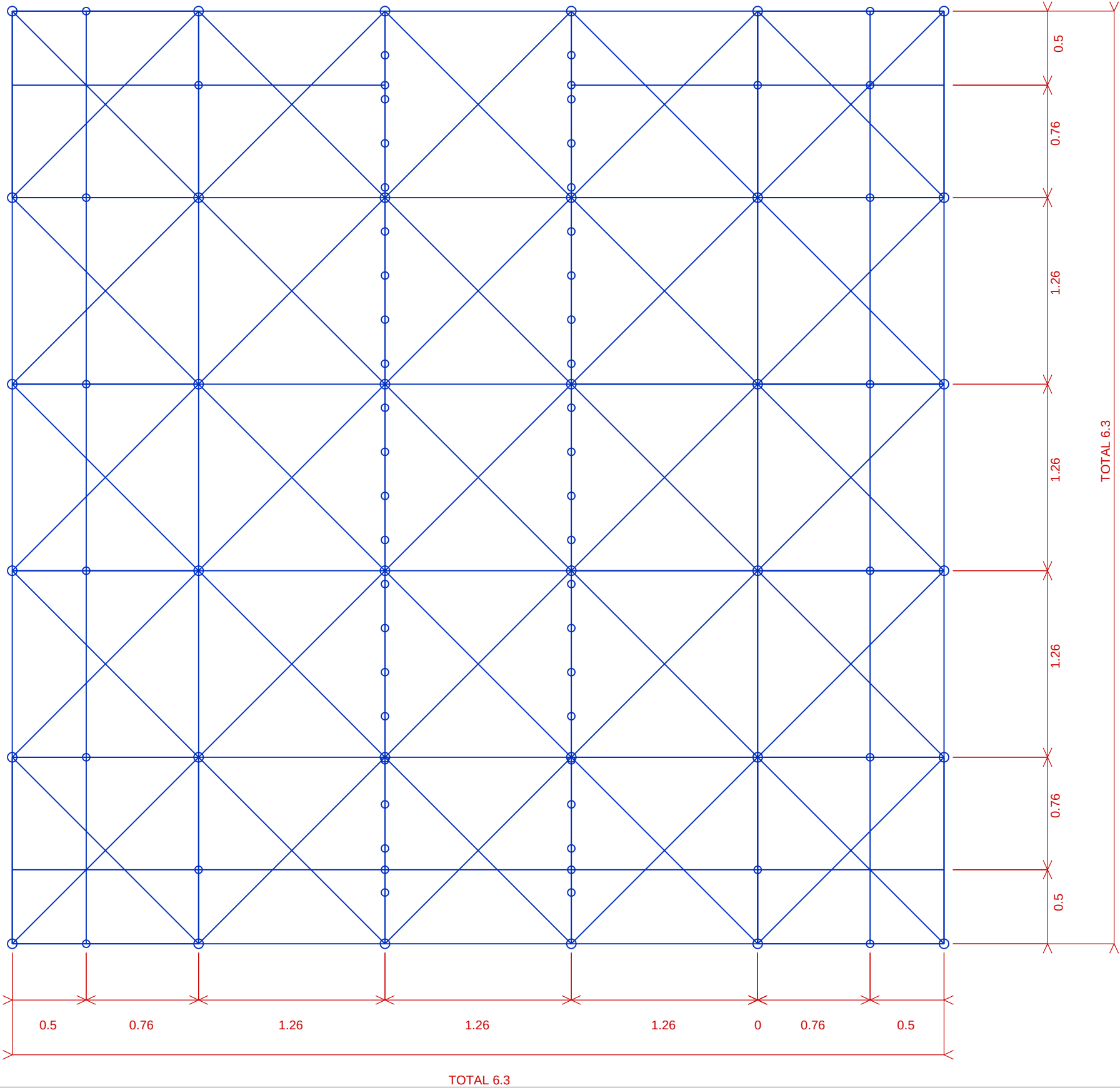
PLAN VIEW
