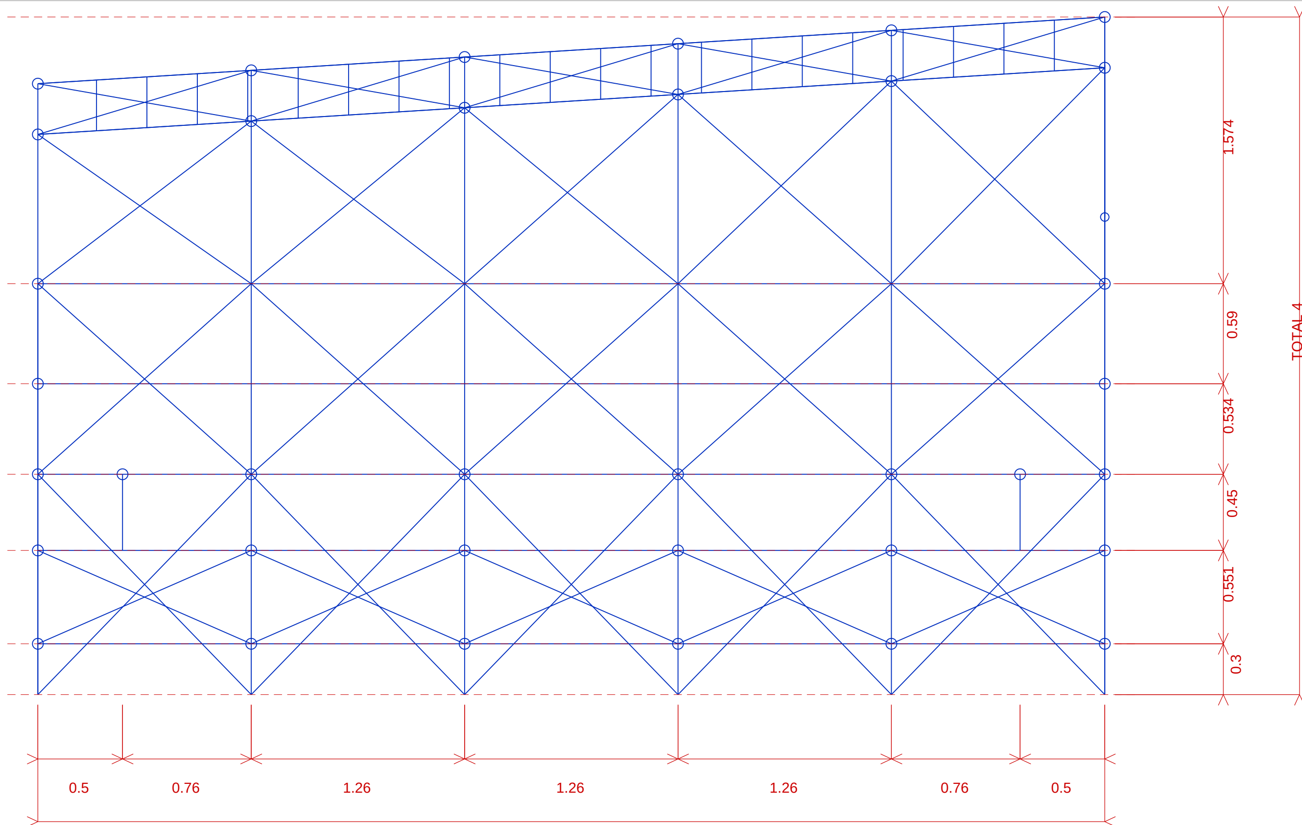
SIDE VIEW
