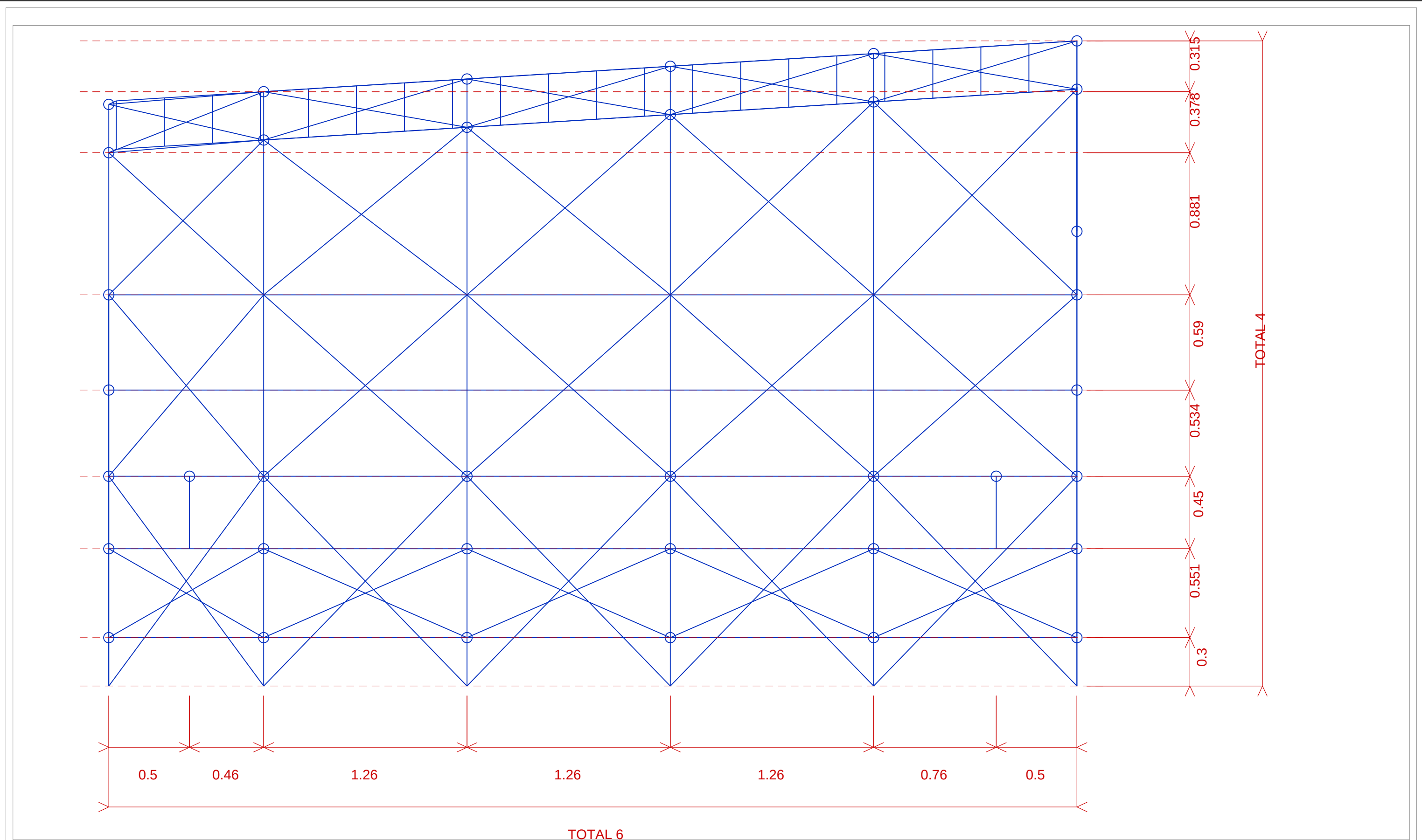
SIDE VIEW
