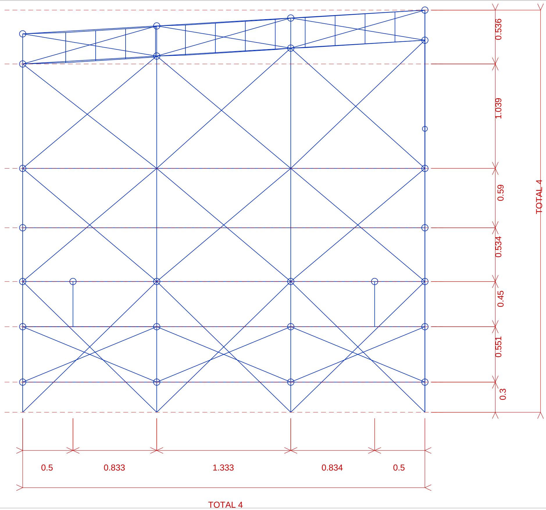
SIDE VIEW
