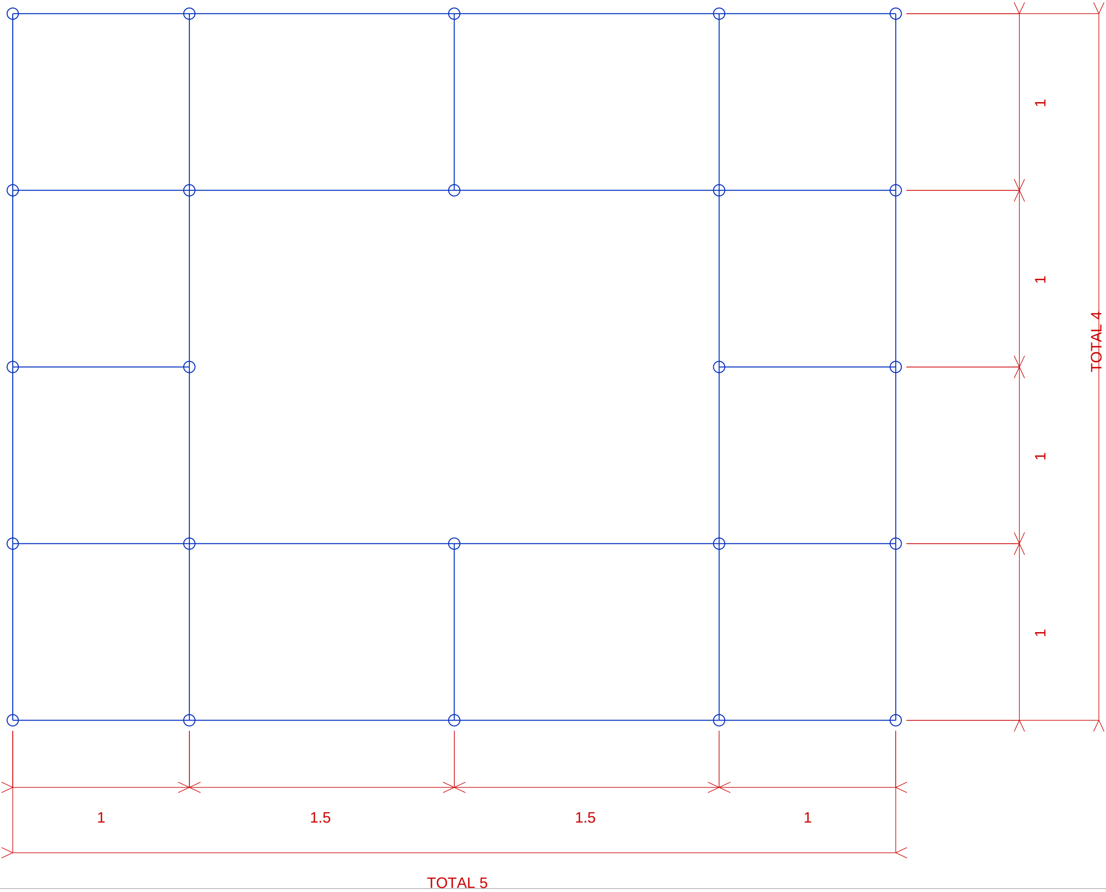
PLAN VIEW
