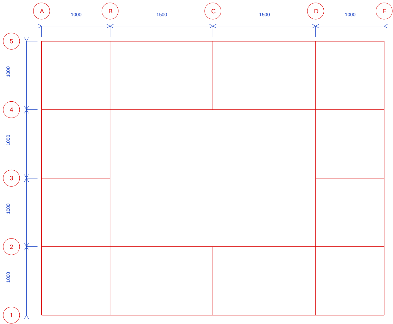
A-FRAME SCAFFOLD PLAN VIEW TYPICAL FOR LEVELS 1, 2, 3, 4, 7, 8, 9, 12, 13, 14, 17, 18, 19, 22, 23 & 24
