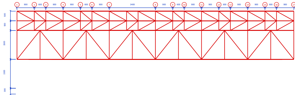
A-FRAME SCAFFOLD FRONT VIEW TYPICAL FOR GRID LINE D (1-17)
