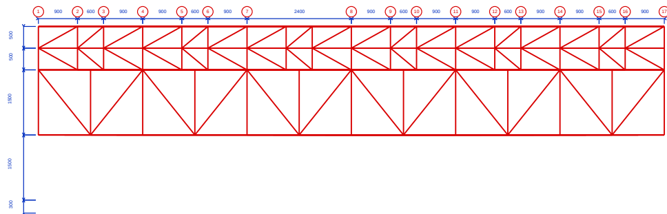
A-FRAME SCAFFOLD FRONT VIEW TYPICAL FOR GRID LINE A (1-17)
