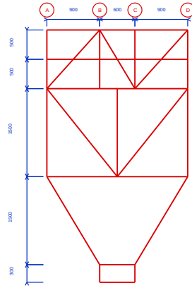
A-FRAME SCAFFOLD SIDE VIEW TYPICAL FOR GRID LINE 1 (A-D)
