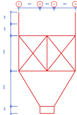
A-FRAME SCAFFOLD SIDE VIEW TYPICAL FOR GRID LINE 4, 7, 8, 11, 14 (A-D)
