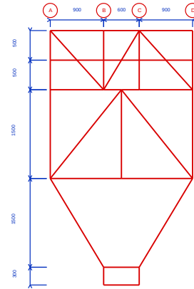
A-FRAME SCAFFOLD SIDE VIEW TYPICAL FOR GRID LINE 17 (A-D)
