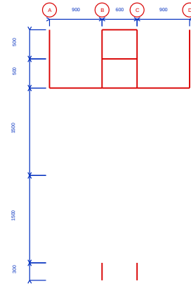
A-FRAME SCAFFOLD SIDE VIEW TYPICAL FOR GRID LINE 2, 3, 5, 6, 9, 10, 12, 13, 15, 16 (A-D)
