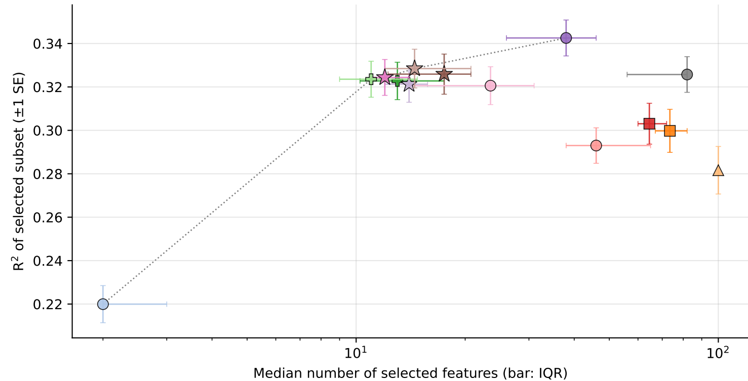
Eye Data, p = 200, n = 120
