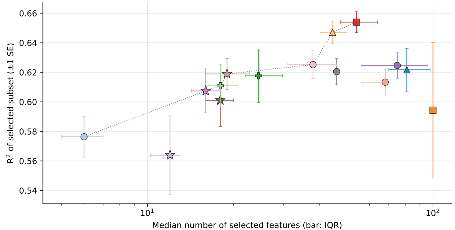
Parkinson's, p = 19, n = 5875
