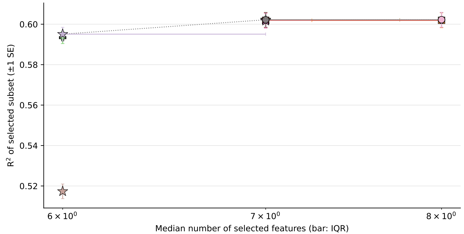
California Housing, p = 8, n = 20640
