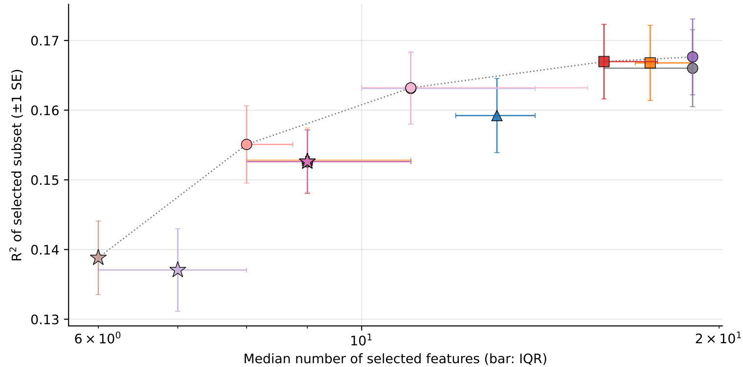
California Housing, p = 8, n = 20640
