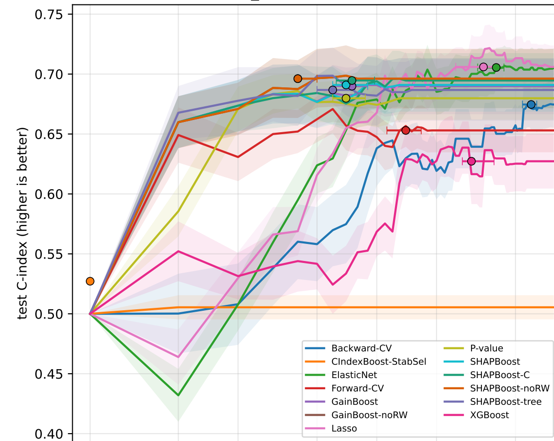
breast_cancer - XGBoost-Cox
