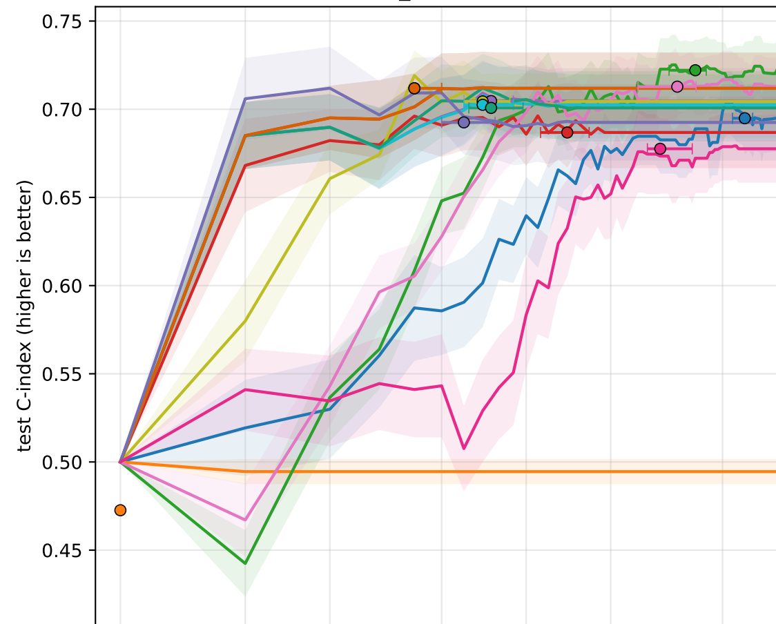
breast_cancer - RSF
