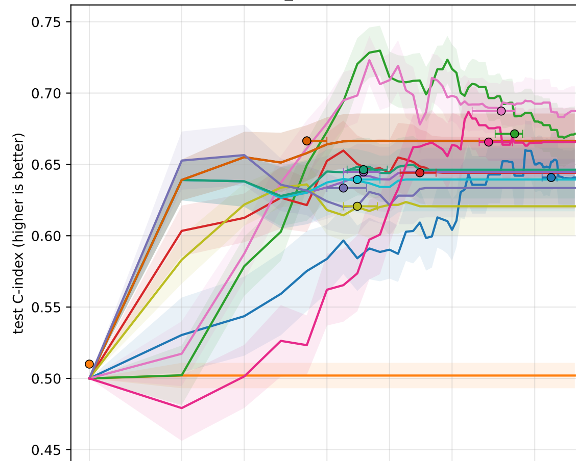
breast_cancer - CoxPH
