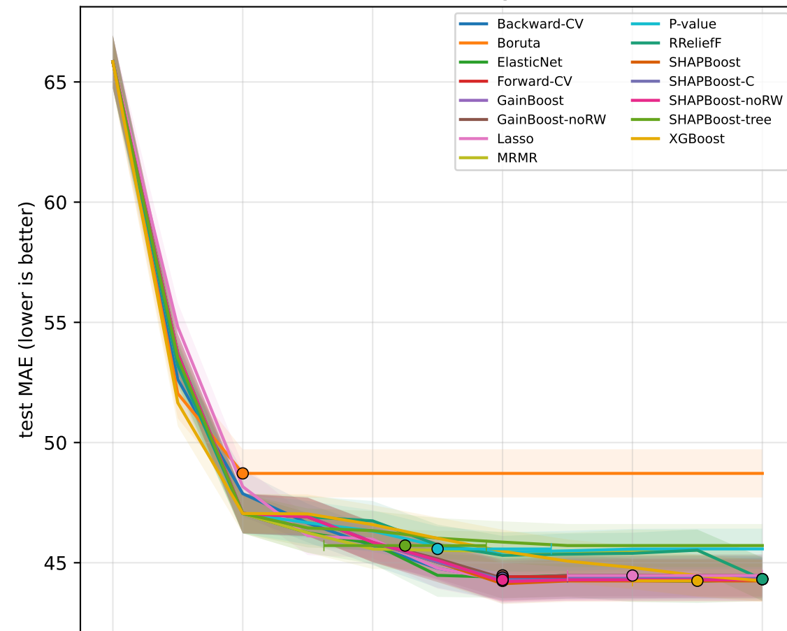
diabetes - LinearRegression
