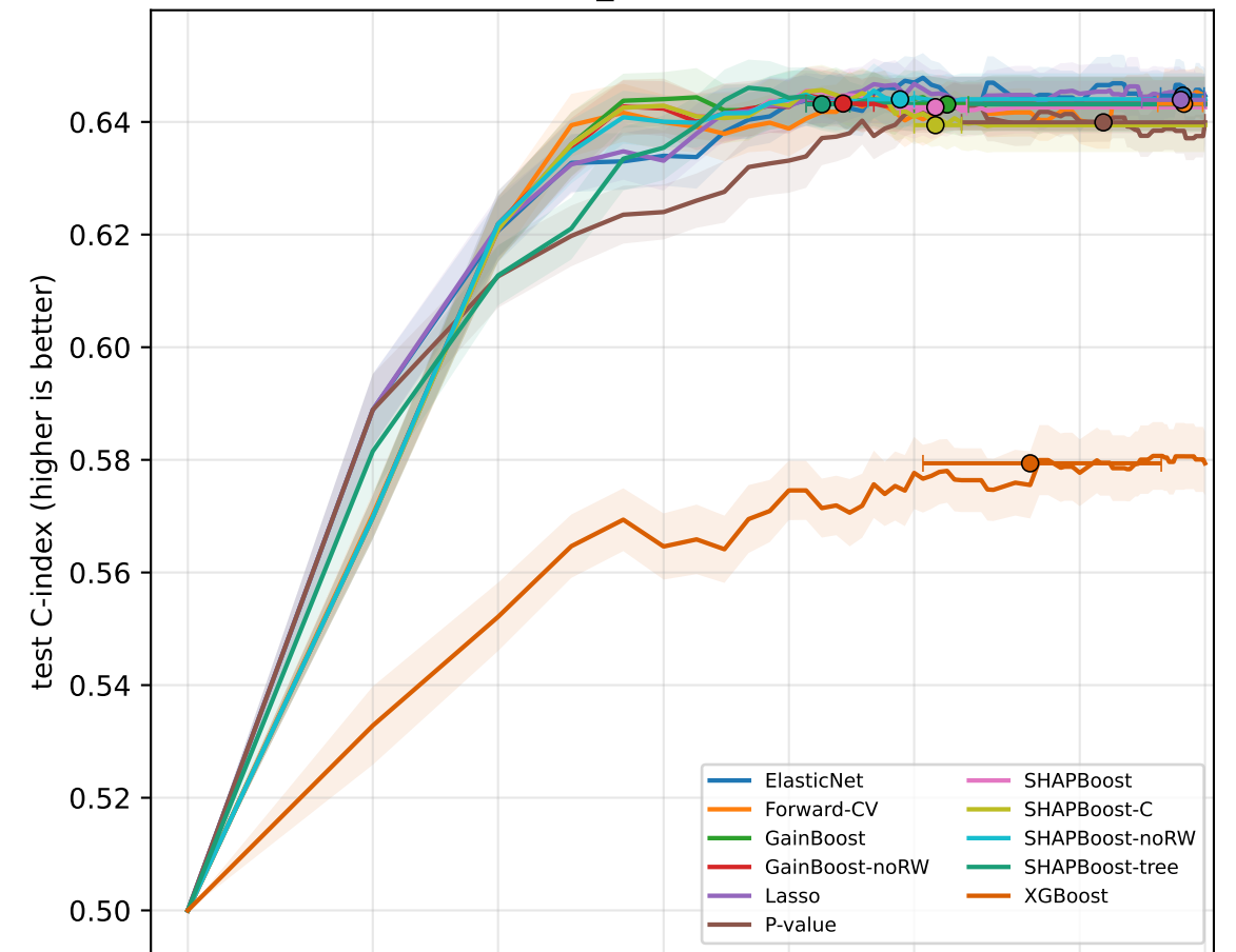
metabric_full - XGBoost-Cox
