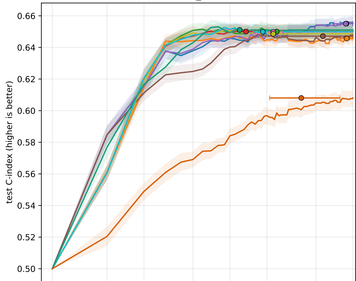
metabric_full - RSF
