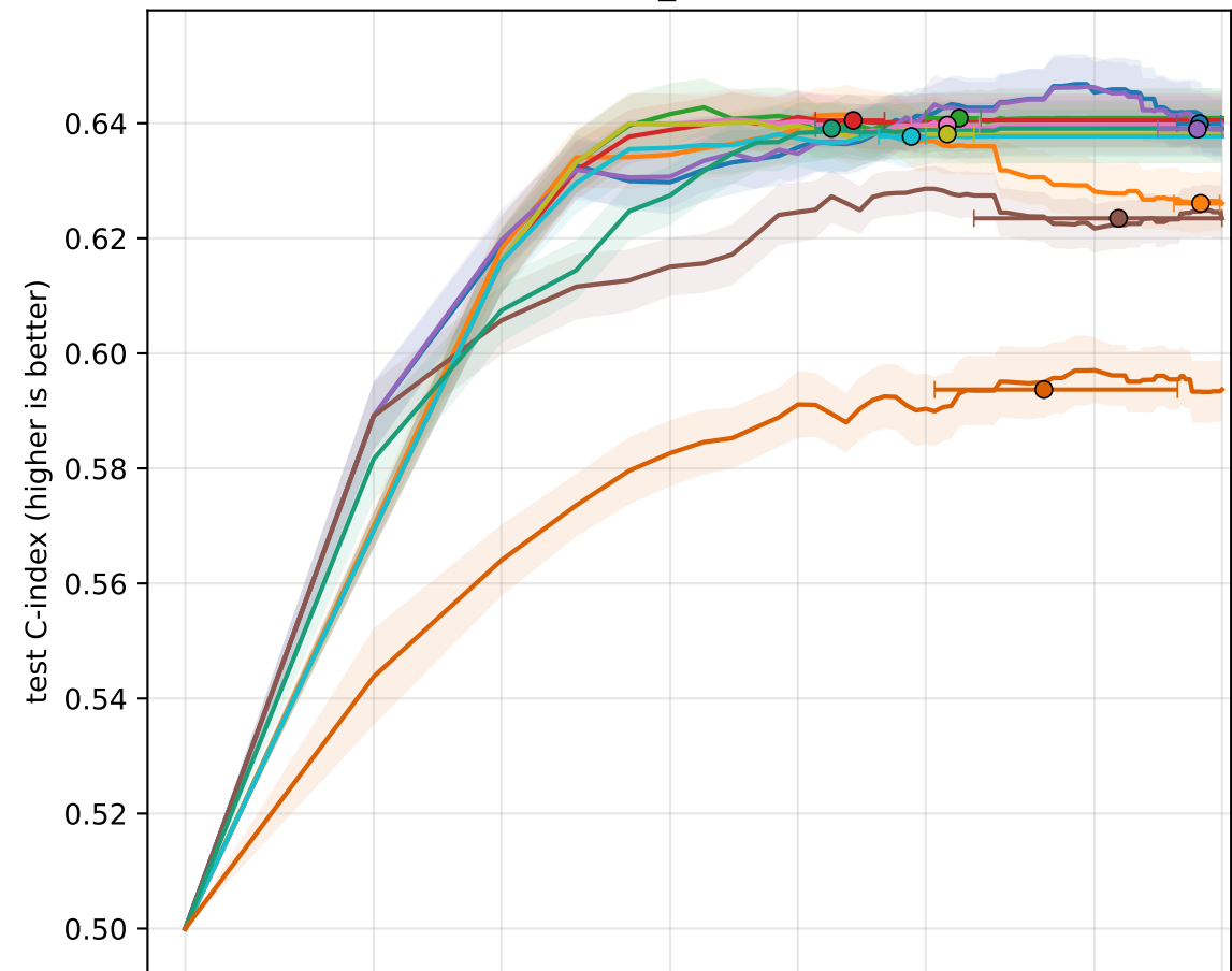
metabric_full - CoxPH
