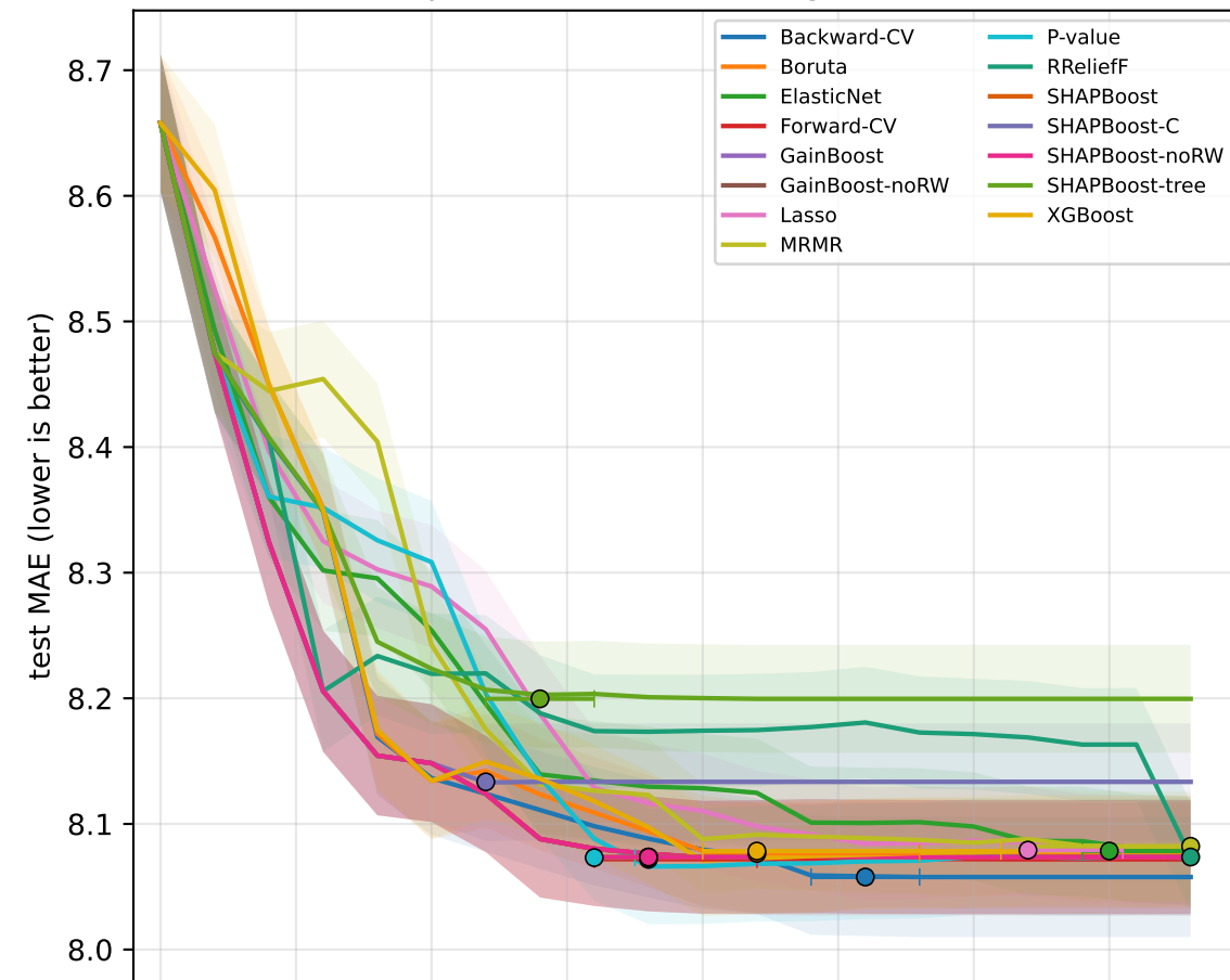
parkinsons - LinearRegression
