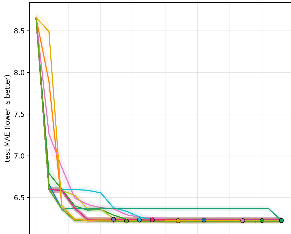
parkinsons - GradientBoosting
