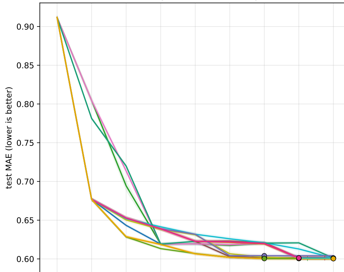
housing - GradientBoosting
