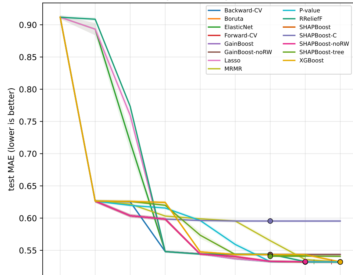
housing - LinearRegression
