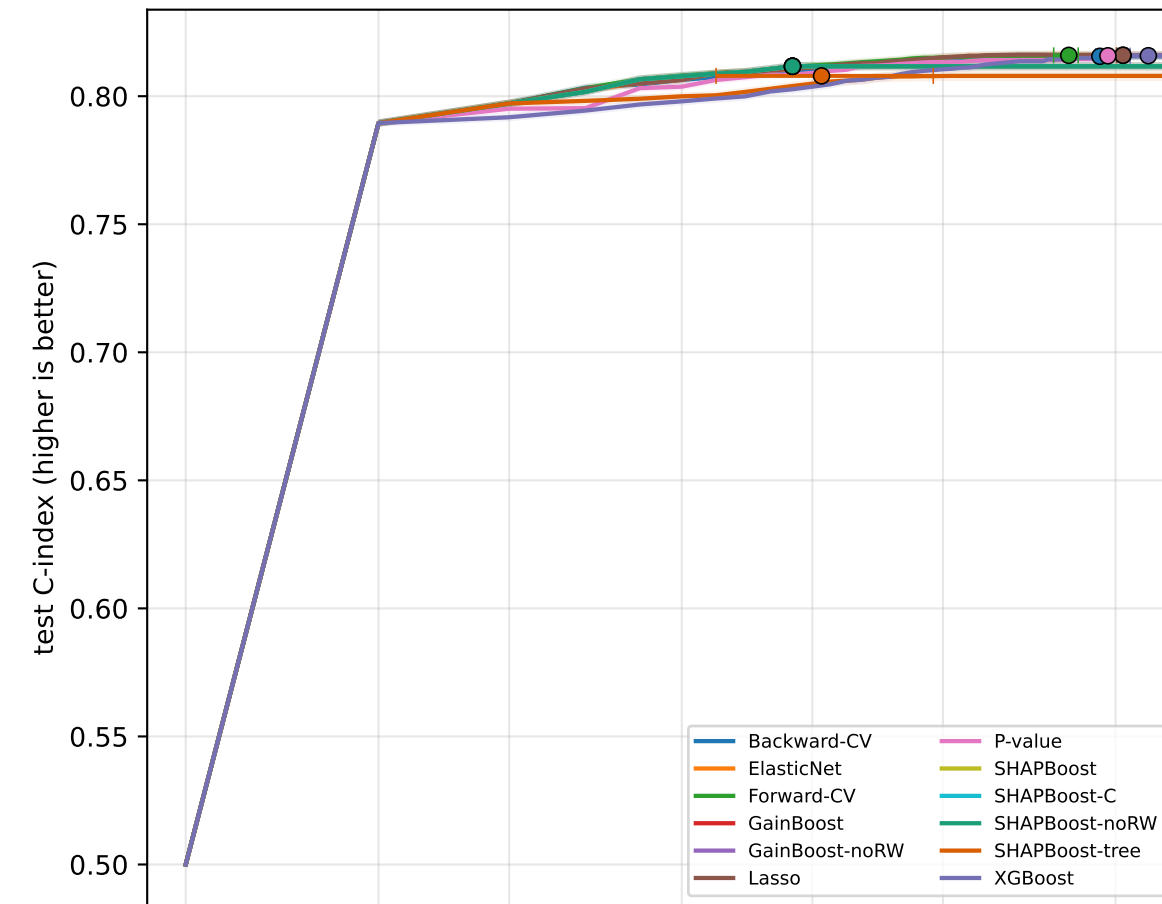
nhanes - XGBoost-Cox
