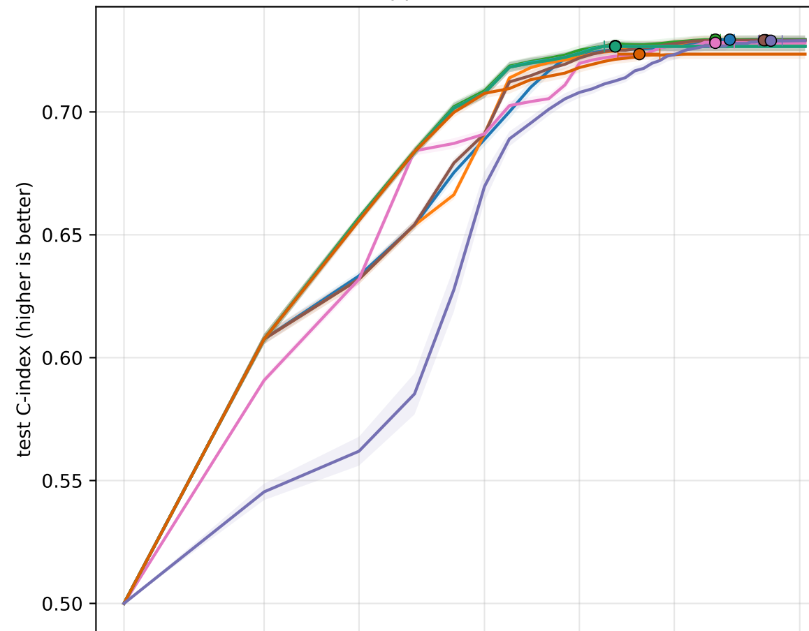
support - CoxPH
