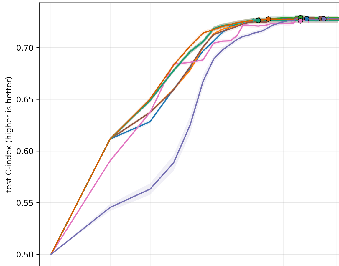
support - RSF
