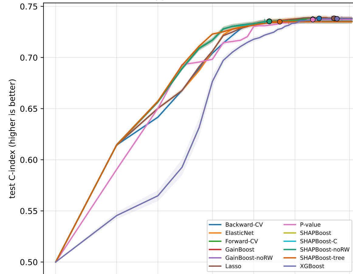
support - XGBoost-Cox
