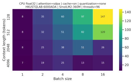
(a) CPU FP32, batches 1–16
