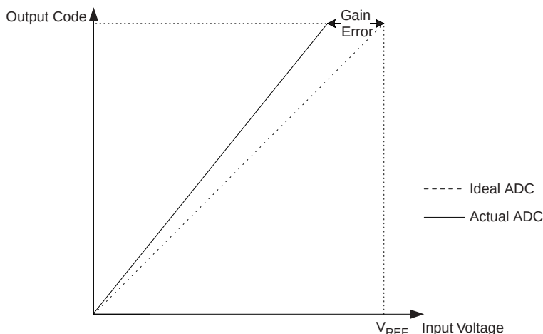
Figure 108. Gain Error
