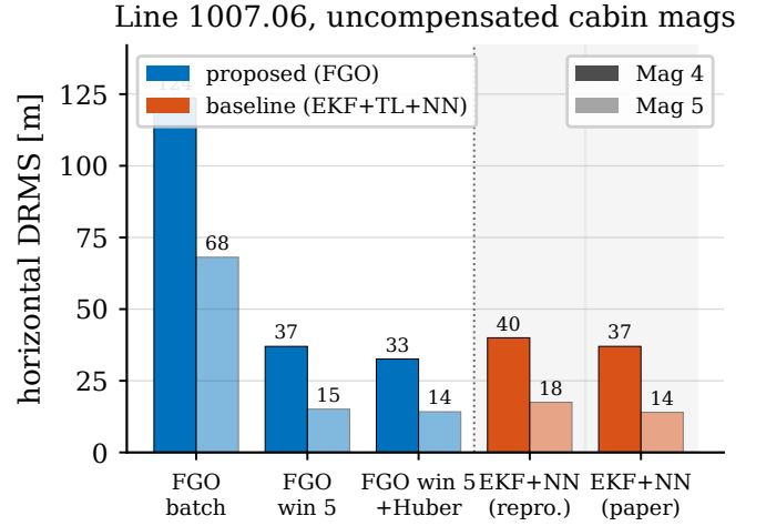
Fig. 9. Line 1007.06 cold start on the uncompensated cabin magnetometers. The NN-free fixed-lag window (left of the divider) matches or beats the reproduced and published EKF+TL+NN (shaded, right).
