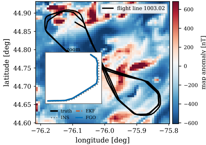
Eastern_395 anomaly map and flight line
