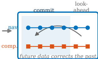
(b) estimate both jointly over a fixed-lag window
