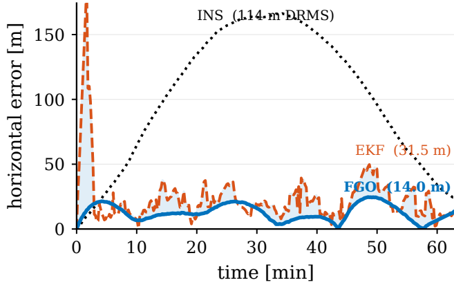
Fig. 6. Horizontal position error on line 1003.02. The batch factor graph (FGO, blue) holds a tighter bound than the EKF (red) across the line; the shaded band marks the FGO improvement, and free inertial (INS) diverges. Legend DRMS values are computed over the full line, without the warm-up exclusion of Table II.
