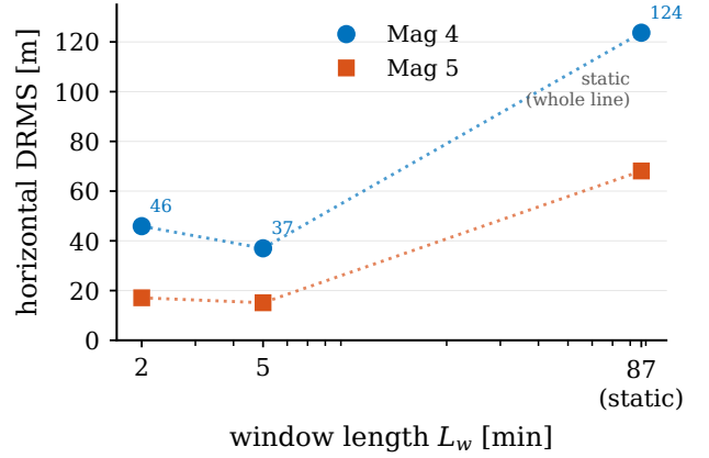
Fig. 8. Window length versus accuracy on line 1007.06 (cold start), at the three evaluated lengths. The 5 min window balances the under-determined 2 min window against the drift-blind static batch (full line).
