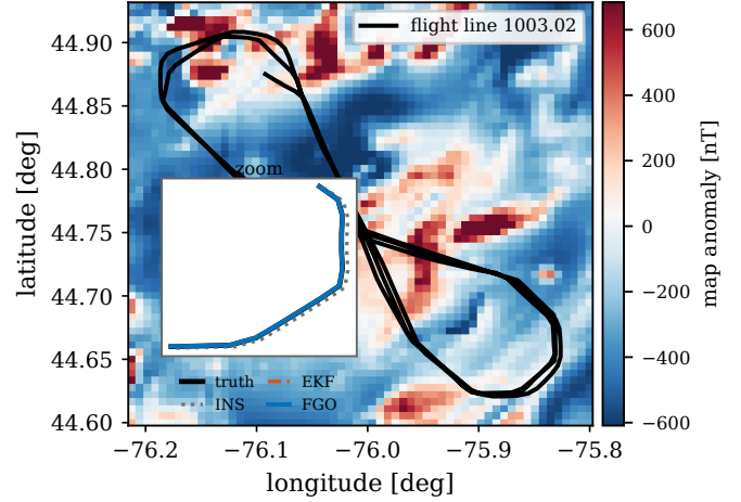
Fig. 5. Eastern anomaly map and flight line 1003.02. The inset zooms a mid-flight window where the free-inertial (INS) track drifts off the truth while the EKF and the factor-graph (FGO) estimates track it.
