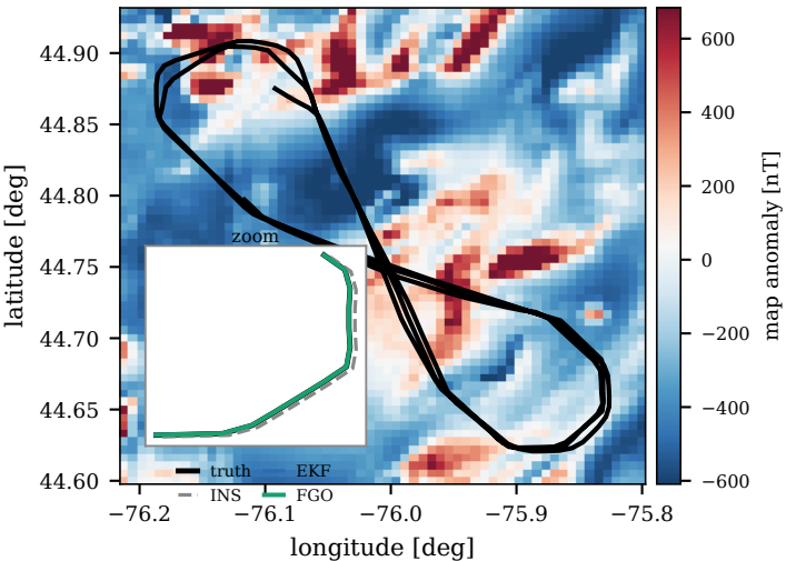
Eastern_395 anomaly map and flight line
