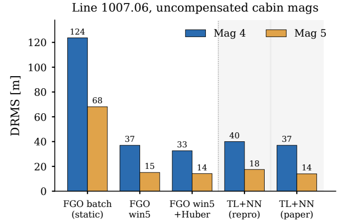
Fig. 5. Line 1007.06 cold start on the uncompensated cabin magnetometers. The NN-free fixed-lag window (left of the divider) matches or beats the reproduced and published EKF+TL+NN (shaded, right).
