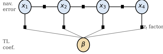
Fig. 1. The Tolles–Lawson coefficient variable \beta is shared by every measurement factor and estimated jointly with the navigation-error chain.
