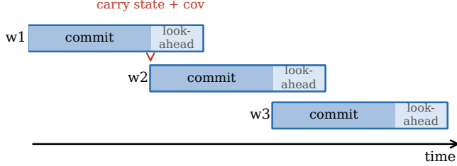
Fig. 2. Each window commits its leading stride and passes the full smoothed state and covariance forward as the prior for the next window.
