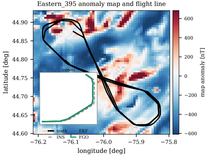
Fig. 3. Eastern anomaly map and flight line 1003.02. The inset zooms a mid-flight window where the free-inertial (INS) track drifts off the truth while the EKF and the factor-graph (FGO) estimates track it.
