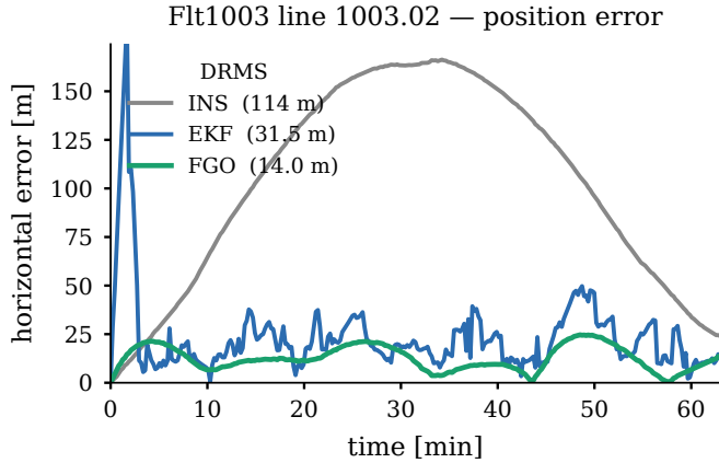
Fig. 4. Horizontal position error on line 1003.02. The batch factor graph (FGO) holds a tighter bound than the EKF across the line; free inertial diverges.
