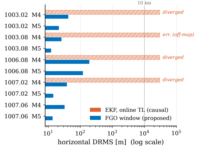
Fig. 10. Breadth study (Table IV) on a log DRMS axis. Hatched bars mark causal EKF divergence beyond 10 km; the fixed-lag window (blue) stays bounded throughout.
