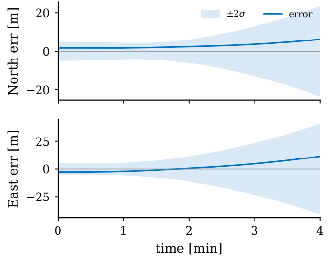
Fig. 13. Covariance envelope. North and East position error for a representative simulated factor-graph run inside the estimator \pm 2\sigma bands. The error stays within the reported uncertainty throughout, consistent with the conservative ANEES of 1.5.
