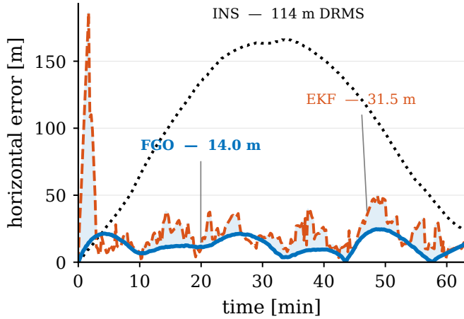
Fig. 7. Horizontal position error on survey line 1003.02 (Flt1003). The batch factor graph (FGO, blue) holds a tighter bound than the EKF (red) across the line; the shaded band marks the FGO improvement, and free inertial (INS) diverges. The labelled DRMS values are computed over the full line, without the warm-up exclusion of Table II.
