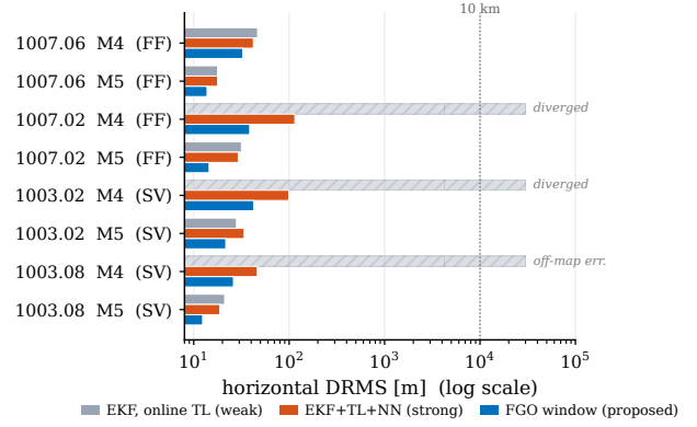
Fig. 10. Breadth study (Table IV) on a log DRMS axis: weak online-TL EKF (gray, hatched where it diverges beyond 10 km), strong EKF+TL+NN (red), and the NN-free FGO window (blue). The NN keeps the causal filter bounded; the window matches that and is best of the three on all 8 full-length cases. The short calibration line 1006.08 is set aside and not shown (see text).
