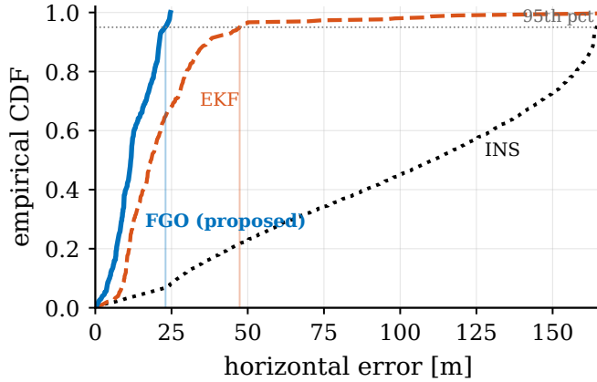
Fig. 7. Empirical CDF of horizontal error on survey line 1003.02 (Flt1003; full line, as in Fig. 6). The proposed FGO reaches its 95th percentile at less than half the EKF's error; both bound the free-inertial error by an order of magnitude.
