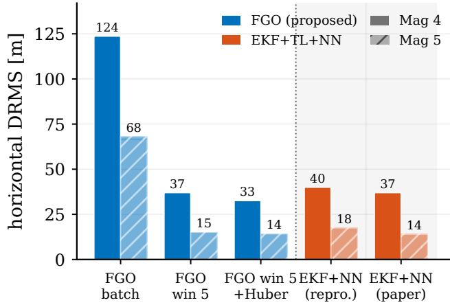
Fig. 9. Free-flight navigation line 1007.06 (Flt1007), cold start on the uncompensated cabin magnetometers. The NN-free fixed-lag window (left of the divider) compares against the reimplemented and reported EKF+TL+NN (shaded, right).
