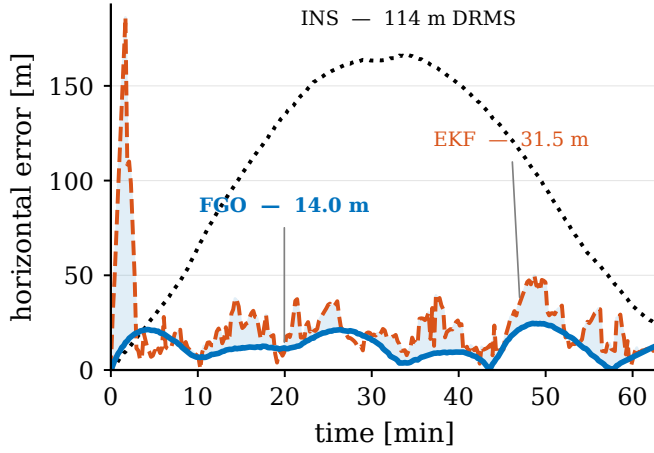
Fig. 6. Horizontal position error on survey line 1003.02 (Flt1003). The batch factor graph (FGO, blue) holds a tighter bound than the EKF (red) across the line; the shaded band marks the FGO improvement, and free inertial (INS) diverges. The labelled DRMS values are computed over the full line, without the warm-up exclusion of Table II.
