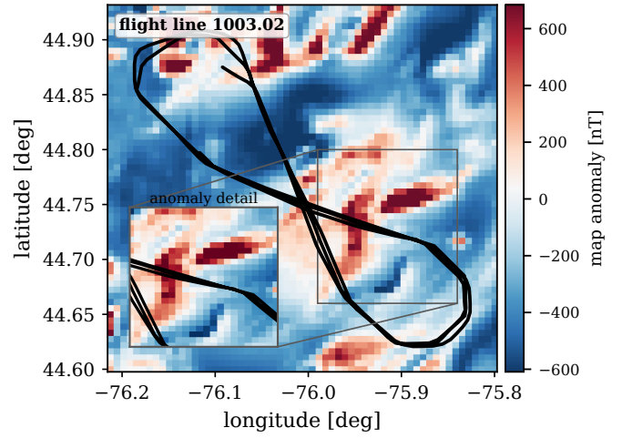
Fig. 5. Eastern anomaly map and survey line 1003.02 (Flt1003 measurement flight), providing geographic context; the inset zooms the fine anomaly structure the map-matching factor exploits along the line. The estimator comparison is deferred to Figs. 6–7: at the survey ground speed a metre-level track error is smaller than one 12 s sample and cannot be resolved on a map.
