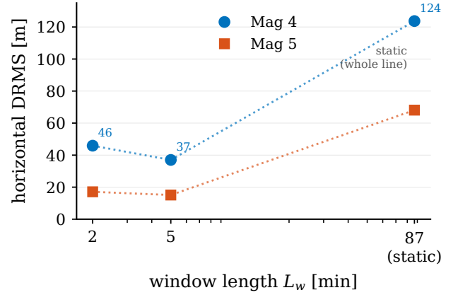
Fig. 8. Window length versus accuracy on the free-flight navigation line 1007.06 (Flt1007, cold start), at the three evaluated lengths. The 5 min window balances the under-determined 2 min window against the drift-blind static batch (full line).
