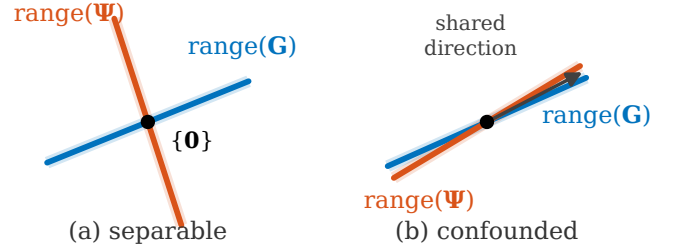
Fig. 5. Observability of joint compensation and navigation (Proposition 1). Left: when the map-gradient subspace \text{range}(\mathbf{G}) and the compensation subspace \text{range}(\Psi) meet only at the origin, position and compensation are separable. Right: when they share a nonzero direction, a position shift can be masked by a compensation change and observability collapses.
