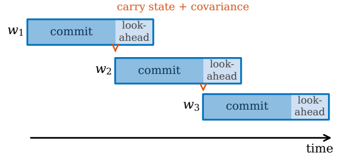
Fig. 4. Fixed-lag sliding window. Each window commits its leading stride and passes the full smoothed state and covariance forward as the prior for the next window; the trailing overlap provides bounded smoother look-ahead.
