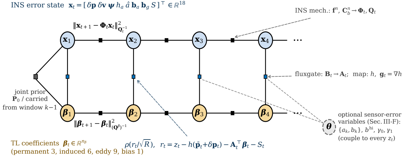
Fig. 3. Factor graph of one window, with every estimated variable and measurement shown. Top: the 18-state INS error chain \mathbf{x}_t of (1), linked by Pinson-FOGM process factors driven by the INS mechanization. Bottom: the time-varying Tolles-Lawson coefficient chain \beta_t , linked by random-walk factors \mathbf{Q}_t . Each scalar-magnetometer factor (blue) applies the robust residual of (8), coupling \delta \mathbf{p}_t , S_t , and \beta_t ; the joint prior (left) is \mathbf{P}_0 at cold start or the covariance carried from the previous window. Dashed arrows mark known factor parameters (INS mechanization, fluxgate basis \mathbf{A}_t , map h, \nabla h ); the dashed node \theta holds the optional sensor-error variables of Section III-F.
