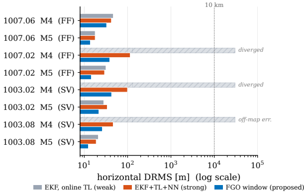
Fig. 11. Breadth study (Table IV) on a log DRMS axis: weak online-TL EKF (gray, hatched where it diverges beyond 10 km), strong EKF+TL+NN (red), and the NN-free FGO window (blue). The NN keeps the causal filter bounded; the window matches that and is best of the three on all 8 full-length cases. The short calibration line 1006.08 is set aside and not shown (see text).
