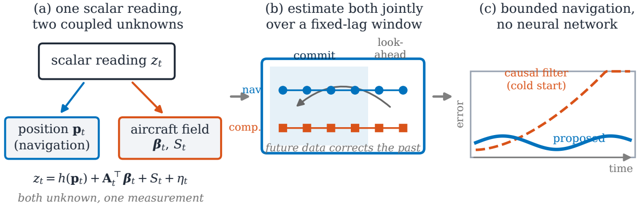
Fig. 1. Concept of the study. (a) A single scalar magnetometer reading mixes the anomaly map signal, which carries the aircraft position \mathbf{p}_t , with the aircraft field, described by the time-varying Tolles–Lawson coefficients \boldsymbol{\beta}_t and a disturbance state S_t ; position and compensation are therefore coupled through the one measurement and must be estimated together. (b) The proposed estimator represents both as variables of a factor graph and solves them jointly over a fixed-lag sliding window, so that measurements after a given epoch still correct its navigation and compensation before the estimate is committed. (c) The result is bounded navigation at cold start, using no neural network, where a causal filter that must commit online can diverge.
