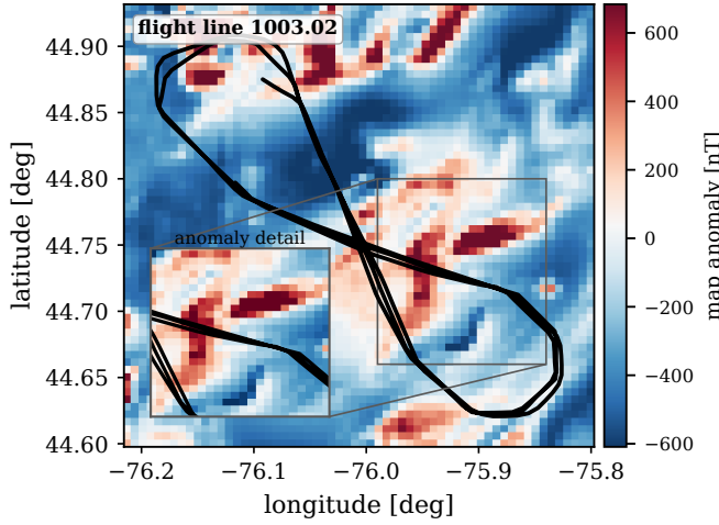
Fig. 6. Eastern anomaly map and survey line 1003.02 (Flt1003 measurement flight), providing geographic context; the inset zooms the fine anomaly structure the map-matching factor exploits along the line. The estimator comparison is deferred to Figs. 7–8: at the survey ground speed a metre-level track error is smaller than one 12 s sample and cannot be resolved on a map.
