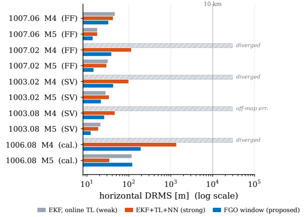
Fig. 10. Breadth study (Table IV) on a log DRMS axis: weak online-TL EKF (gray, hatched where it diverges beyond 10 km), strong EKF+TL+NN (red), and the NN-free FGO window (blue). The NN keeps the causal filter bounded; the window matches that and is best of the three on all 8 full-length cases (the 14 min line 1006.08 is excluded as its post-warm-up window is too short to compare).
