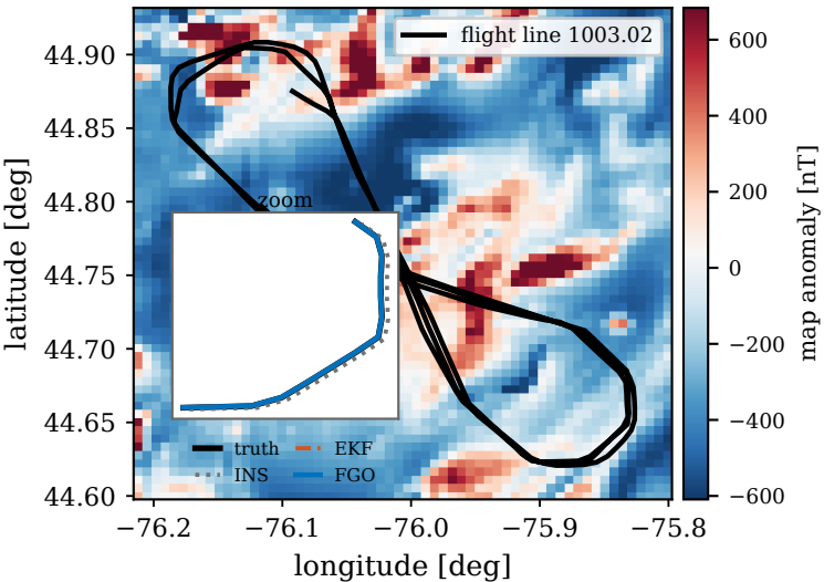
Eastern_395 anomaly map and flight line
