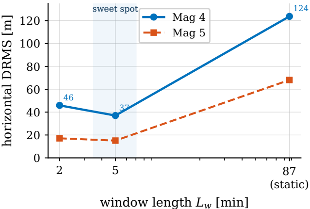
Window length vs accuracy, line 1007.06
