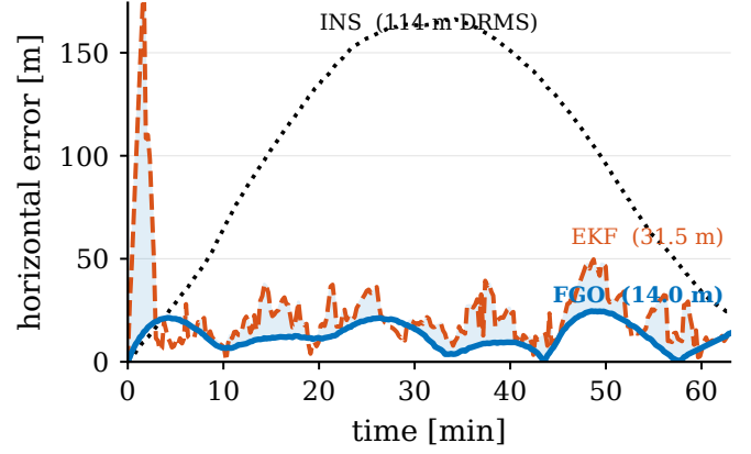
Fig. 6. Horizontal position error on line 1003.02. The batch factor graph (FGO, blue) holds a tighter bound than the EKF (red) across the line; the shaded band marks the FGO improvement, and free inertial (INS) diverges. Legend DRMS values are computed over the full line, without the warm-up exclusion of Table II.
