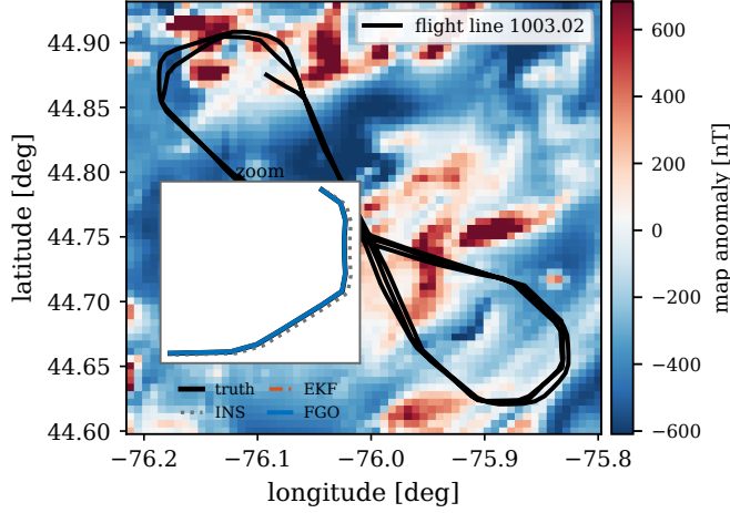
Fig. 5. Eastern anomaly map and flight line 1003.02. The inset zooms a mid-flight window where the free-inertial (INS) track drifts off the truth while the EKF and the factor-graph (FGO) estimates track it.
