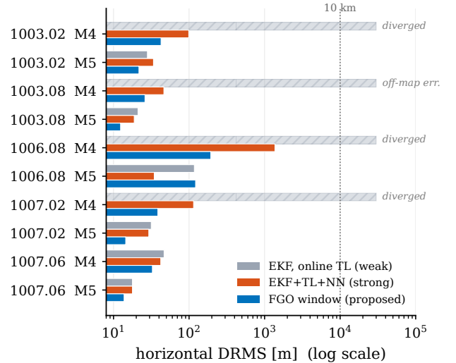
Fig. 10. Breadth study (Table IV) on a log DRMS axis: weak online-TL EKF (gray, hatched where it diverges beyond 10 km), strong EKF+TL+NN (red), and the NN-free FGO window (blue). The NN keeps the causal filter bounded; the window matches that and is best of the three on all 8 full-length cases (the 14 min line 1006.08 is excluded as its post-warm-up window is too short to compare).
