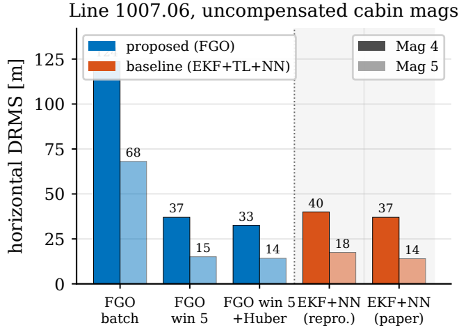
Fig. 7. Line 1007.06 cold start on the uncompensated cabin magnetometers. The NN-free fixed-lag window (left of the divider) matches or beats the reproduced and published EKF+TL+NN (shaded, right).
