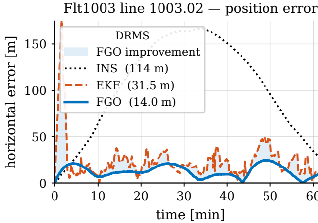
Fig. 5. Horizontal position error on line 1003.02. The batch factor graph (FGO, blue) holds a tighter bound than the EKF (red) across the line; the shaded band marks the FGO improvement, and free inertial (INS) diverges.
