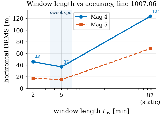
Fig. 8. Window length versus accuracy on line 1007.06 (cold start). A 5 min window is the sweet spot between the under-determined 2 min window and the drift-blind static batch (full line).
