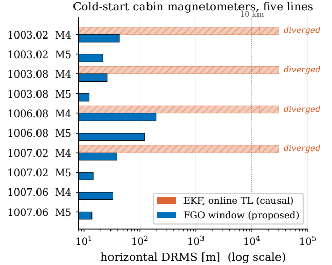
Fig. 10. Breadth study (Table III) on a log DRMS axis. Hatched bars mark causal EKF divergence beyond 10 km; the fixed-lag window (blue) stays bounded throughout.
