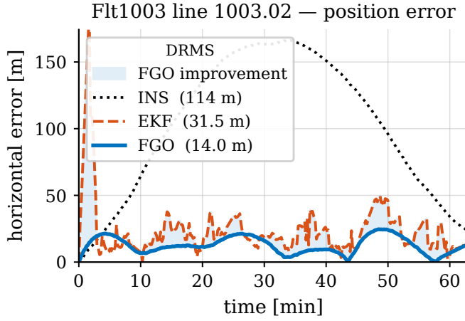
Fig. 6. Horizontal position error on line 1003.02. The batch factor graph (FGO, blue) holds a tighter bound than the EKF (red) across the line; the shaded band marks the FGO improvement, and free inertial (INS) diverges.
