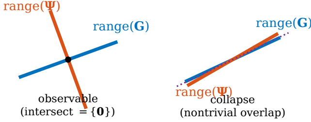
Fig. 4. Observability of joint compensation and navigation (Proposition 1). Left: when the map-gradient subspace \text{range}(\mathbf{G}) and the compensation subspace \text{range}(\Psi) meet only at the origin, position and compensation are separable. Right: when they share a nonzero direction, a position shift can be masked by a compensation change and observability collapses.
