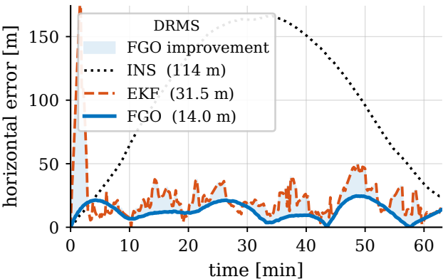
Flt1003 line 1003.02 — position error
