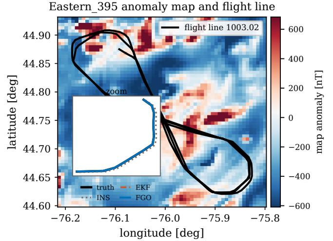
Fig. 4. Eastern anomaly map and flight line 1003.02. The inset zooms a mid-flight window where the free-inertial (INS) track drifts off the truth while the EKF and the factor-graph (FGO) estimates track it.
