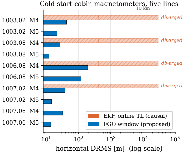
Fig. 8. Breadth study (Table II) on a log DRMS axis. Hatched bars mark causal EKF divergence beyond 10 km; the fixed-lag window (blue) stays bounded throughout.
