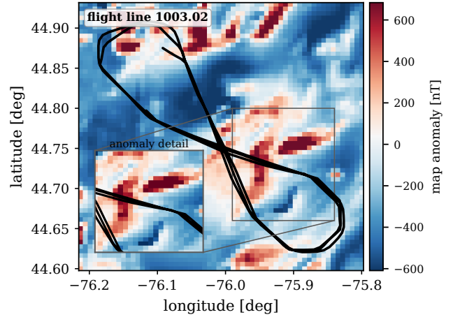
Fig. 6. Eastern anomaly map and survey line 1003.02 (Flt1003 measurement flight), providing geographic context; the inset zooms the fine anomaly structure the map-matching factor exploits along the line. The estimator comparison is deferred to Figs. 7–8: at the survey ground speed a metre-level track error is smaller than one 12 s sample and cannot be resolved on a map.
