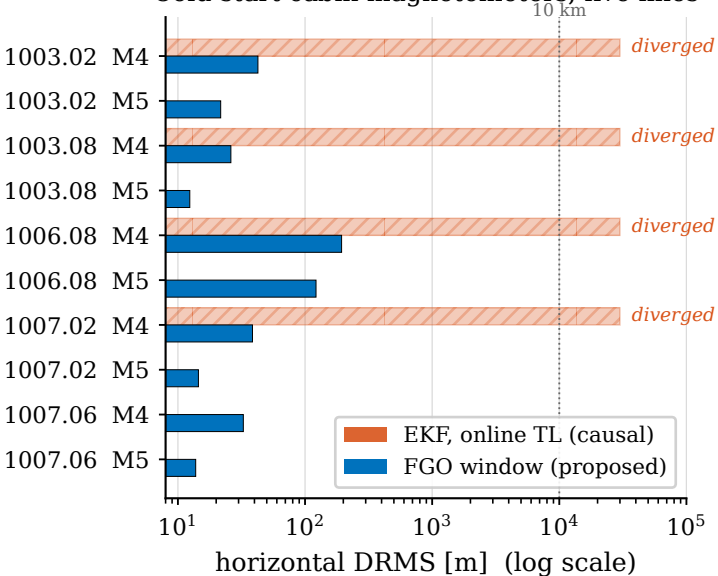
Cold-start cabin magnetometers, five lines
