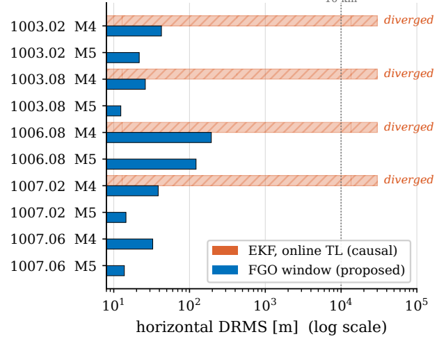
Cold-start cabin magnetometers, five lines
