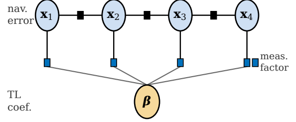
Fig. 2. Factor graph. The Tolles–Lawson coefficient variable \beta (shared, bottom) enters every measurement factor and is estimated jointly with the navigation-error chain \mathbf{x}_1, \dots, \mathbf{x}_N .
