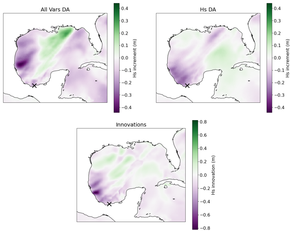
FIGURE 5.3: Significant wave height ensemble mean increments at 12Z 12/03/2022 from all vars DA (top left) and H_s DA (top right), and significant wave height innovations from the same time (bottom). Taken from 12Z 10/03/2022 forecast run. The buoy location is marked with a cross.
